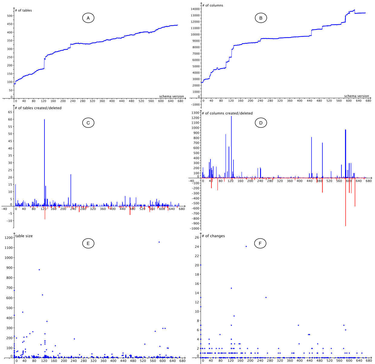
Figure 3: Extracted information from the OSCAR historical schema: (A) evolution of the number of tables; (B) evolution of the number of columns; (C) creation/deletion of tables; (D) creation/deletion of columns; (E) table creation version VS table size; (F) table creation version VS number of changes;.
