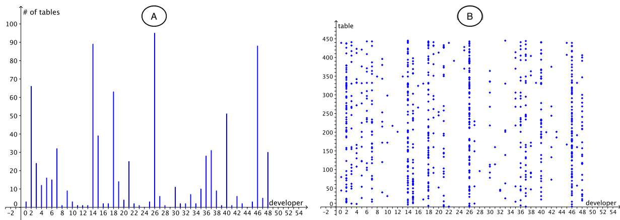
Figure 4: Information about the developers involved in the evolution of the OSCAR database schema. (A) number of tables impacted by each developer; (B) table vs developer matrix.
