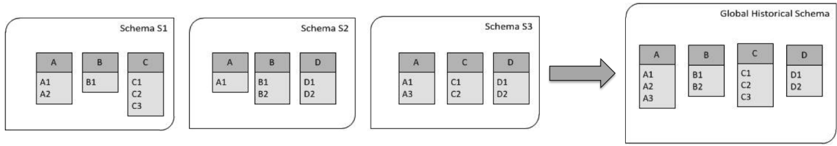
Figure 1: Schema evolution example (left) and corresponding historical schema (right)
